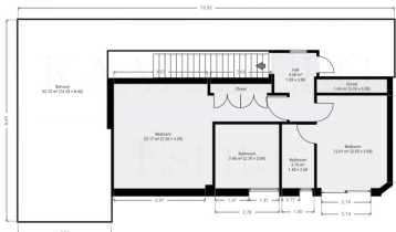
NOT TO SCALE 1st floor
